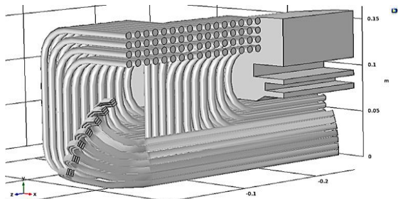
Fig. 6. Cutaway isometric view of the flared-end region of the windings.
