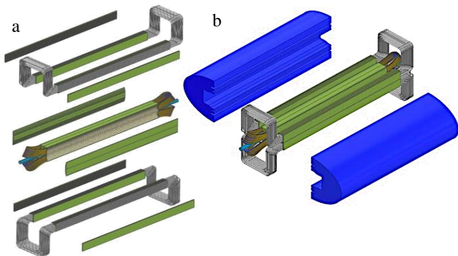
Fig. 5. Blow-up illustration of the winding and assembly of the hybrid dipole. a) The outsert winding is fabricated as two halves while the insert is fabricated; b) The outsert is then assembled with Inconel supports (green) around the insert winding, the flux returns are slid on, and preload is applied.
