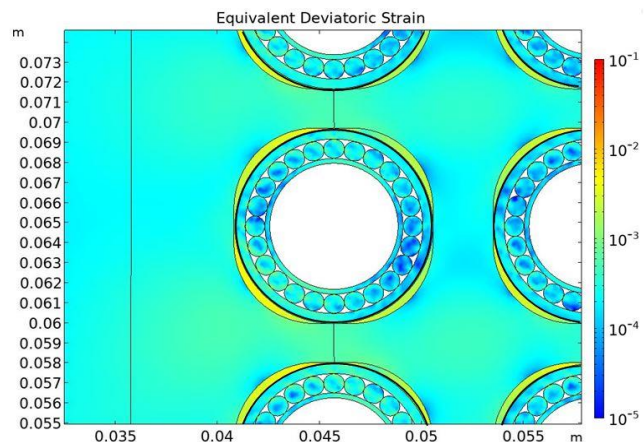
Fig. 12. Simulated deviatoric strain distribution in the CIC winding turn with greatest stress. Insulating S-2 fiberglass sock (black) is pulled over the sheath tube.
