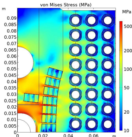
Fig. 10. Distribution of von Mises stress in the hybrid dipole at 18.5 T.
